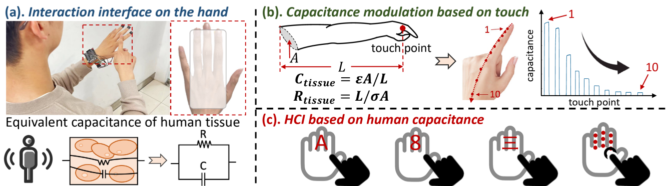
Figure 1: A taste of HandPad : (a) Our bodies can be constructed as capacitive circuits. (b) When we touch different locations on one hand with a finger from the other, the intrinsic capacitance of our arm is altered. (c) Utilizing changes in human capacitance during touch interactions, we engineer a skin-based touchscreen system that supports multiple input modalities.
